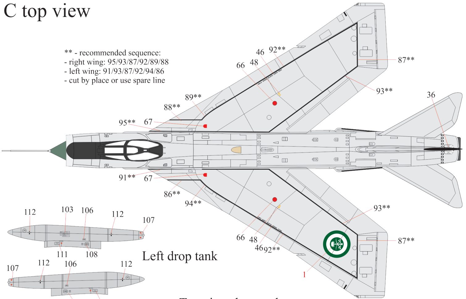
Top view drop tank
