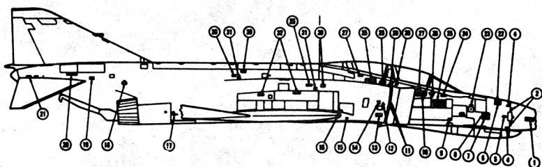
FUSELAGE RIGHT SIDE
