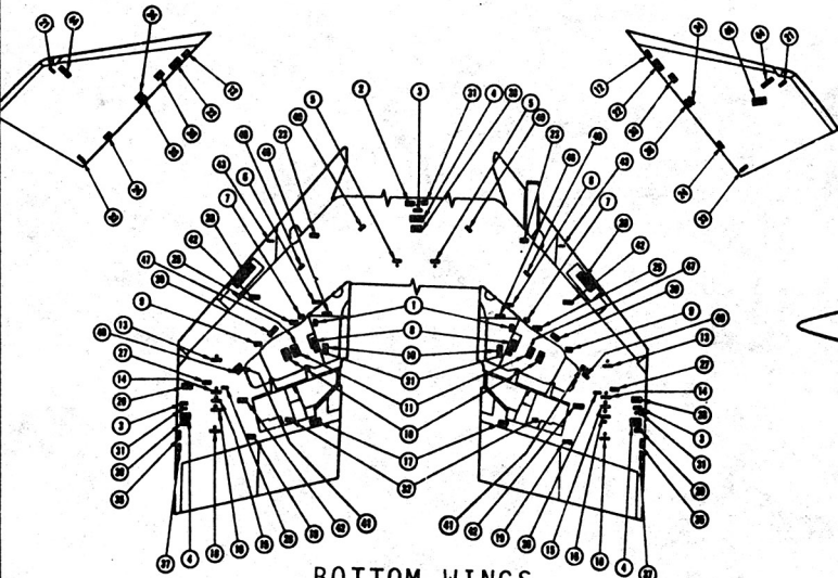
BOTTOM WINGS
