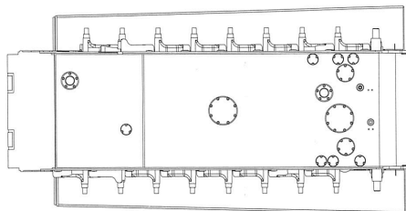
Lower Hull
