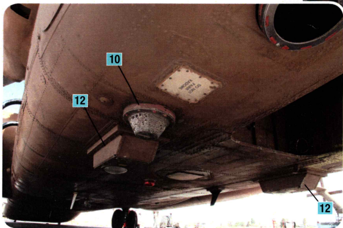
Formation lights location
