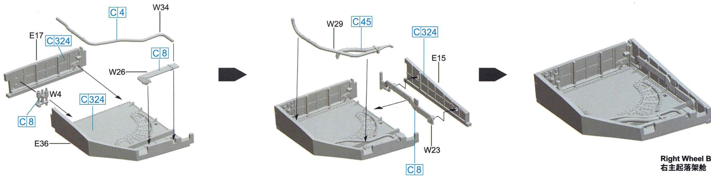
Left Wheel Bay 左主起落架舱
