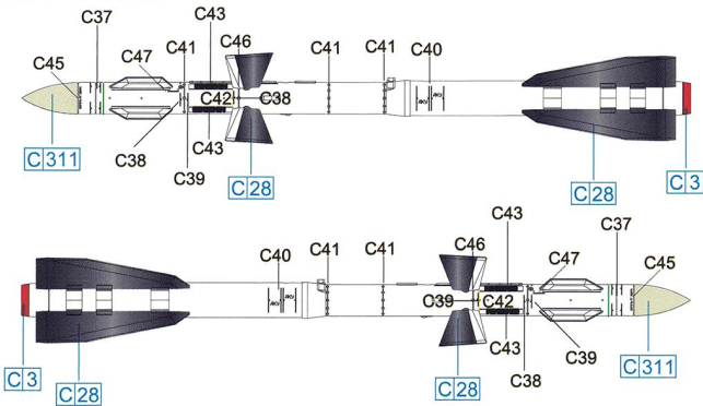
R-27ER "AA-10" Missile R-27ER "AA-10" 空空导弹
