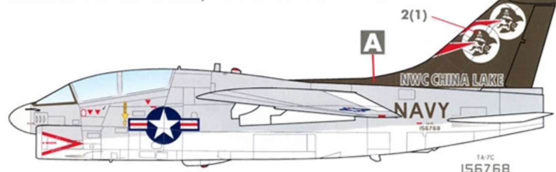
OPTION 3: TA-7C BU.NO. 156768, NAVAL WEAPONS CENTER - CHINA LAKE
