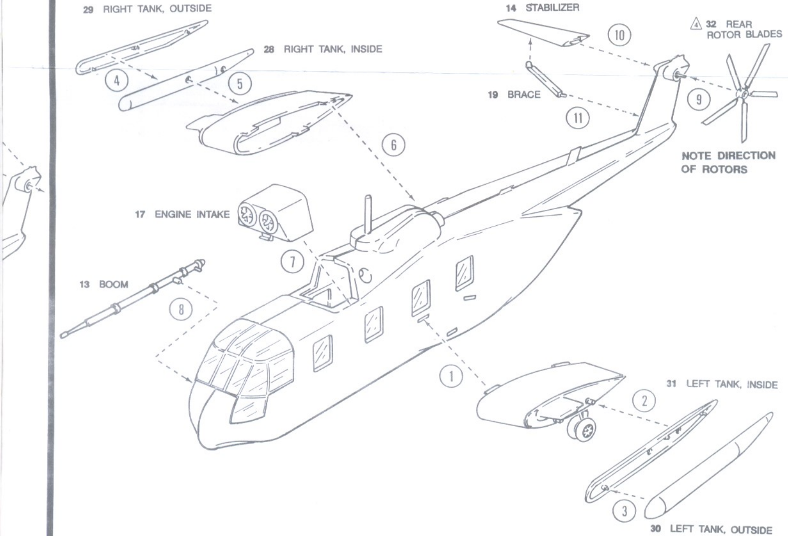
14 STABILIZER
