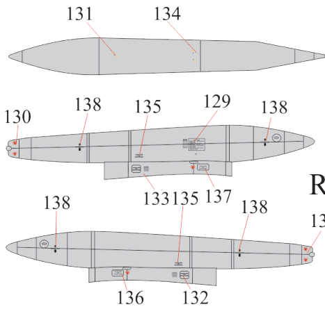
Top view drop tank
