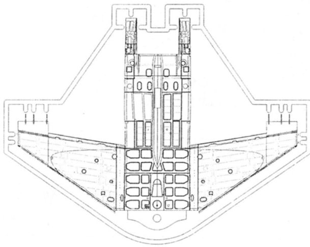
Upper fuselage
