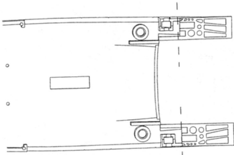
Upper Fuselage
