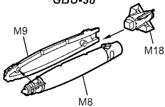
GBU-38
