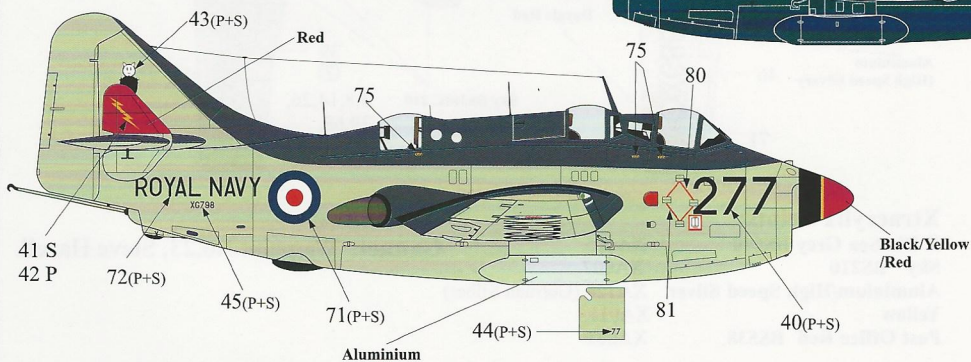
Fairey Gannet ECM.Mk6, XG798., 831 Sqn. FAA, RNAS Culdrose, 1963.
