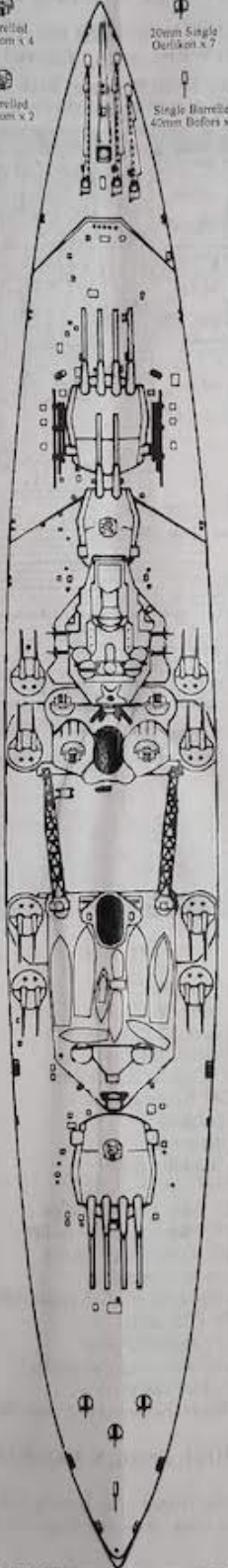
HMS Prince of Wales Late 1941 AA Armament Plan
