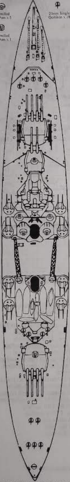
HMS King George V Late 1941 AA Armament Plan
