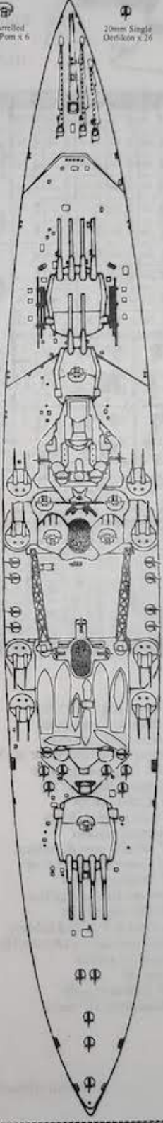
HMS Duke of York Mid 1943 AA Armament Plan
