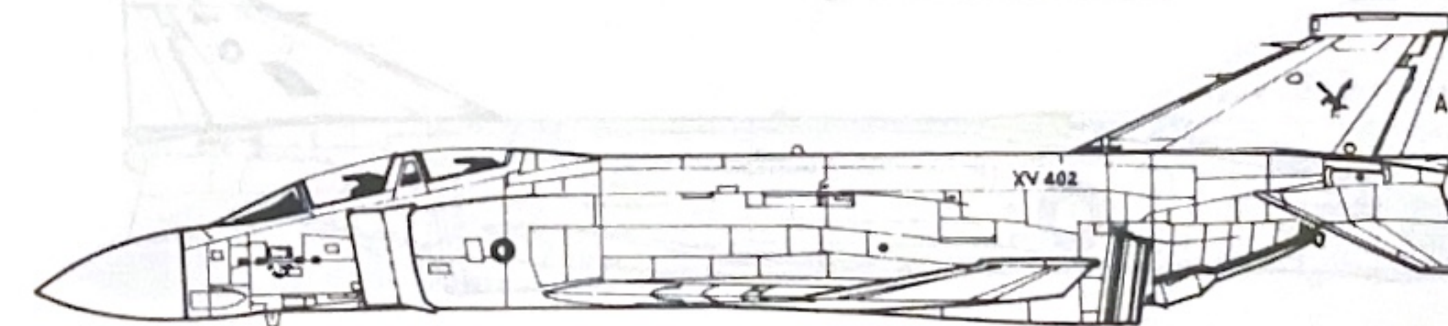
FGR.2 23 Sqn (Falkland Is) 1985 XV 402 'A' Low-viz scheme
