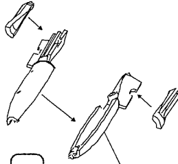
WEAPON SET A MK82
