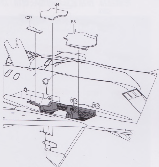
左轮舱关闭状态 Main landing gear bay in the left closing state
