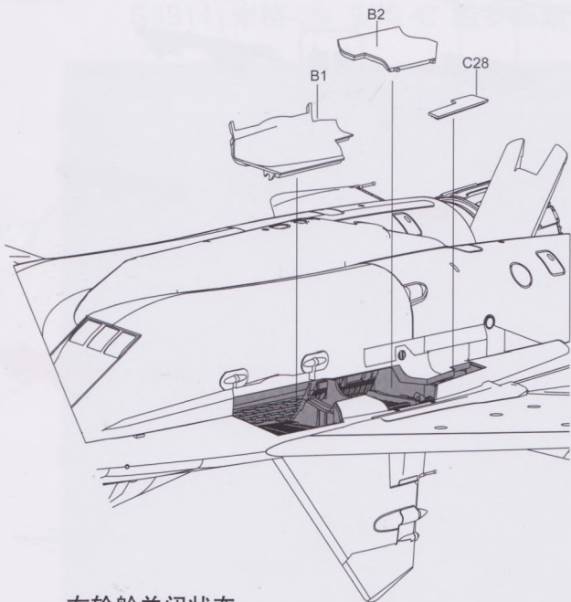
右轮舱关闭状态 Main landing gear bay in the right closing state
