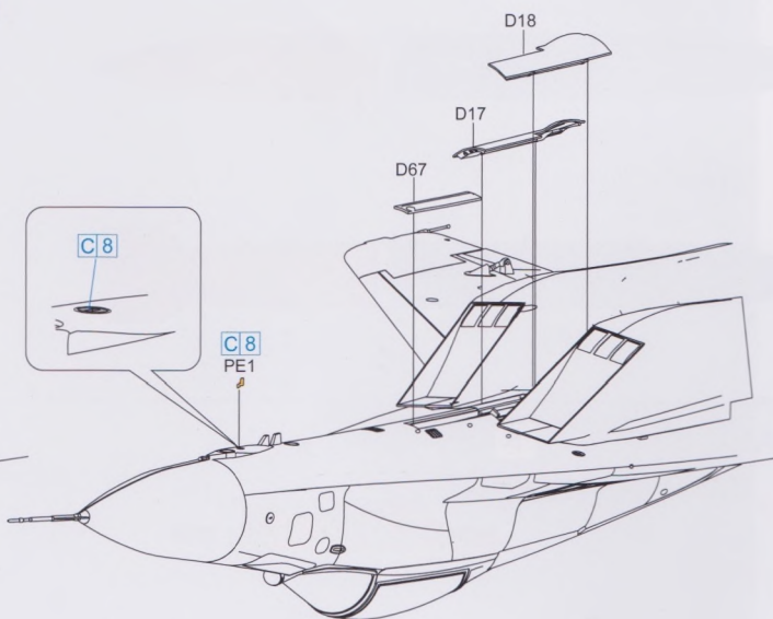
前轮舱关闭状态 Front landing gear bay closing state
