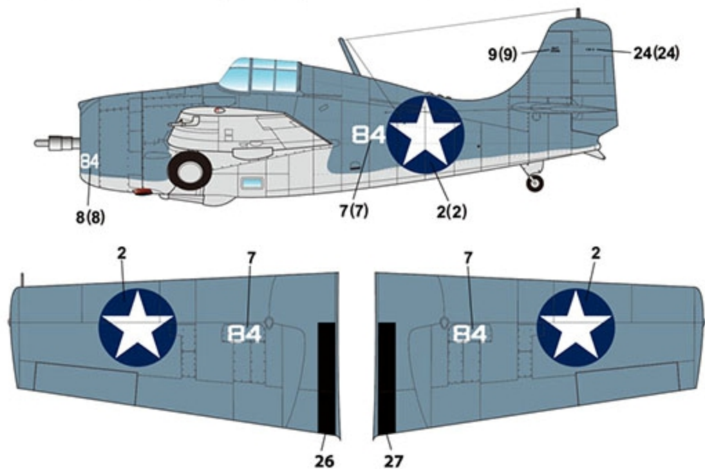
1. F4F-4 BuNo. Unknown/white 84, flown by Captain Joseph Jacob Foss, VMF-121, USMC, Henderson Field, Guadalcanal, Oct. 1942
