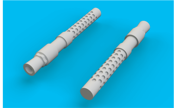
648 402 Bf 109G-6 exhaust stacks
