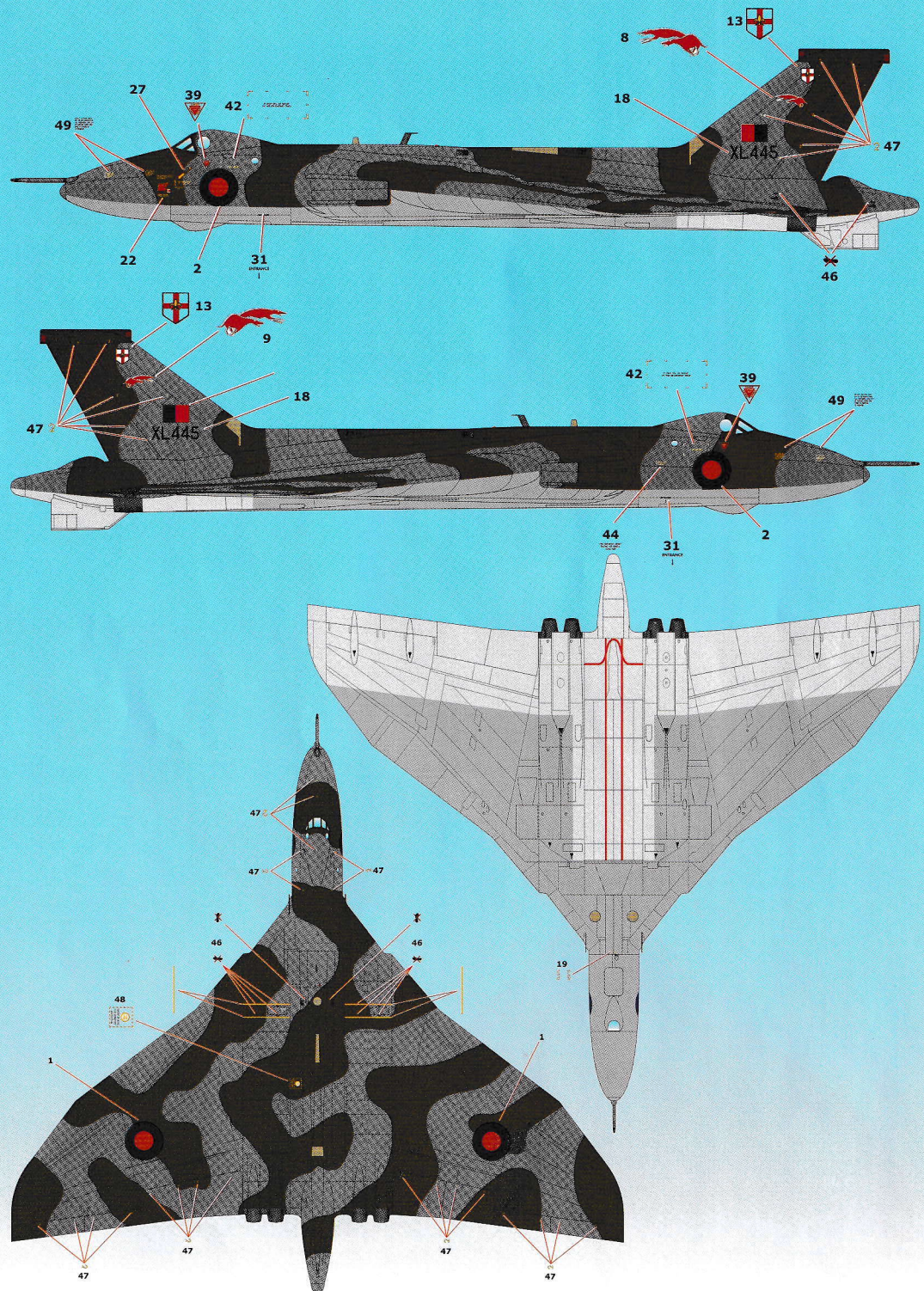
(3) Avro Vulcan K.2 Tanker, XL445, 50th Sqn. Waddington, England, UK, Mar. 1984
