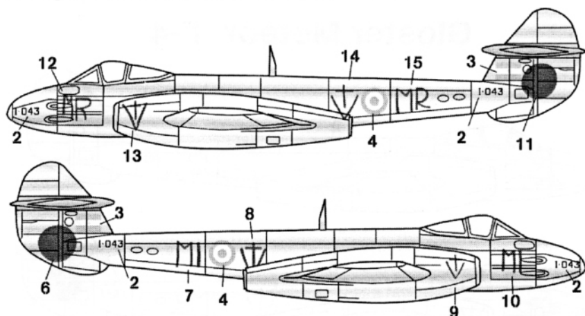
Gloster Meteor F4 C-005, "Grupo Aereo 7" BAM Moron, early 1970
