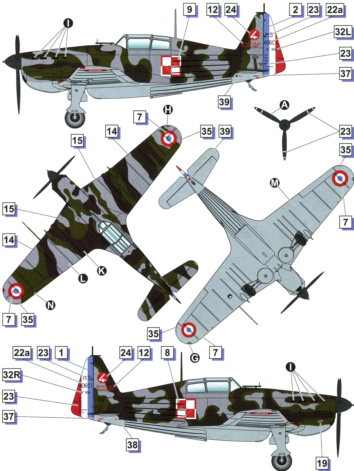
MS.406 №906, pilot Cpl. Edward Uchto, Fighter Training Flight, DIAP Lyon-Bron, June 1940
