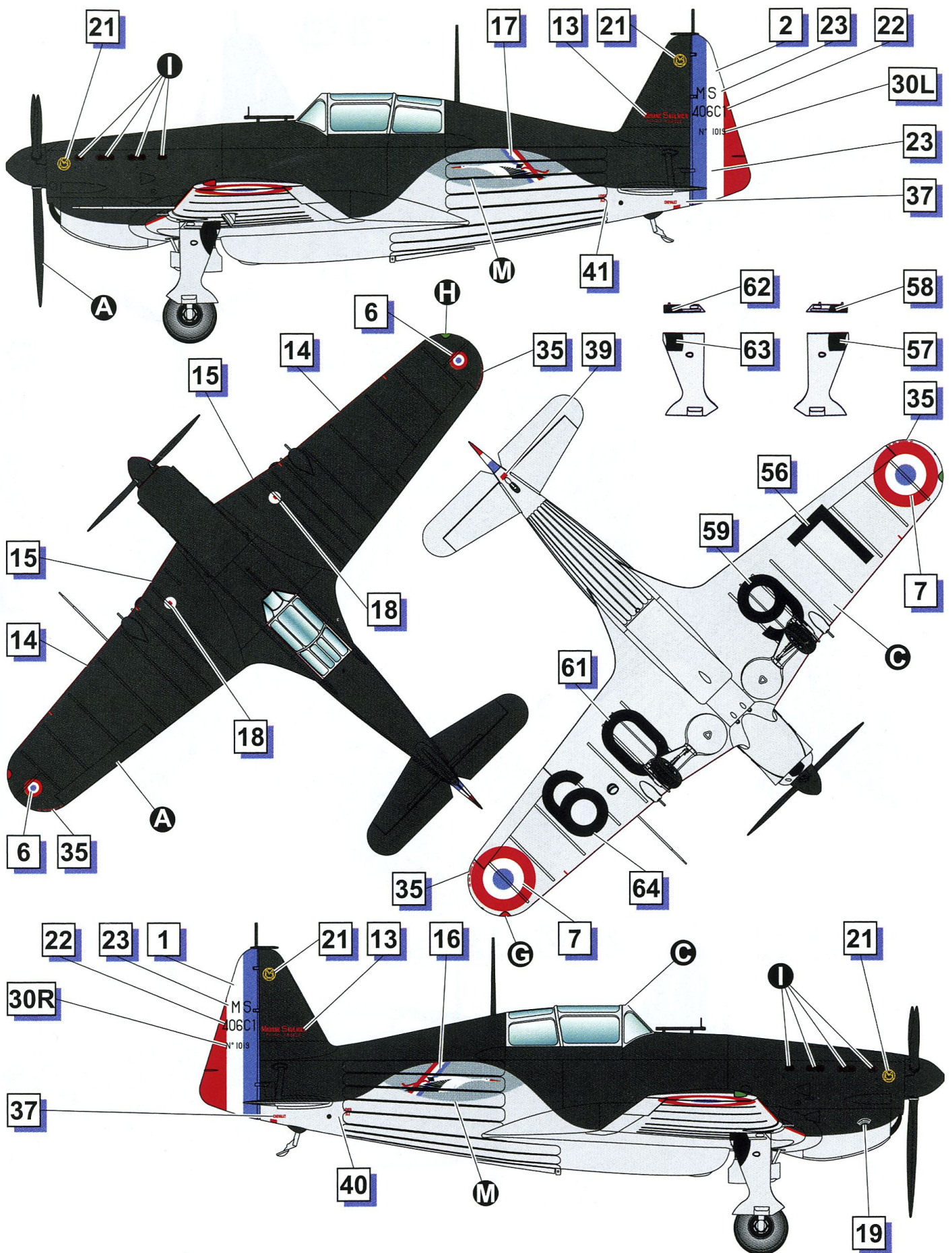
MS.406 №1019, named "Le Pirate". Personal airplane General Armand Pinsard (27 victories in WW1), Commandant Groupment de Chasse 21, May 1940
