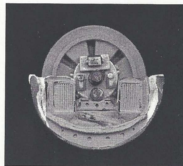
Assembled Heat Exchanger / Center Section
