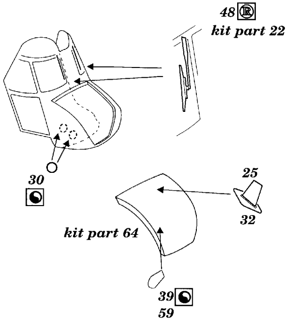
CH-47D -USAF version - late
