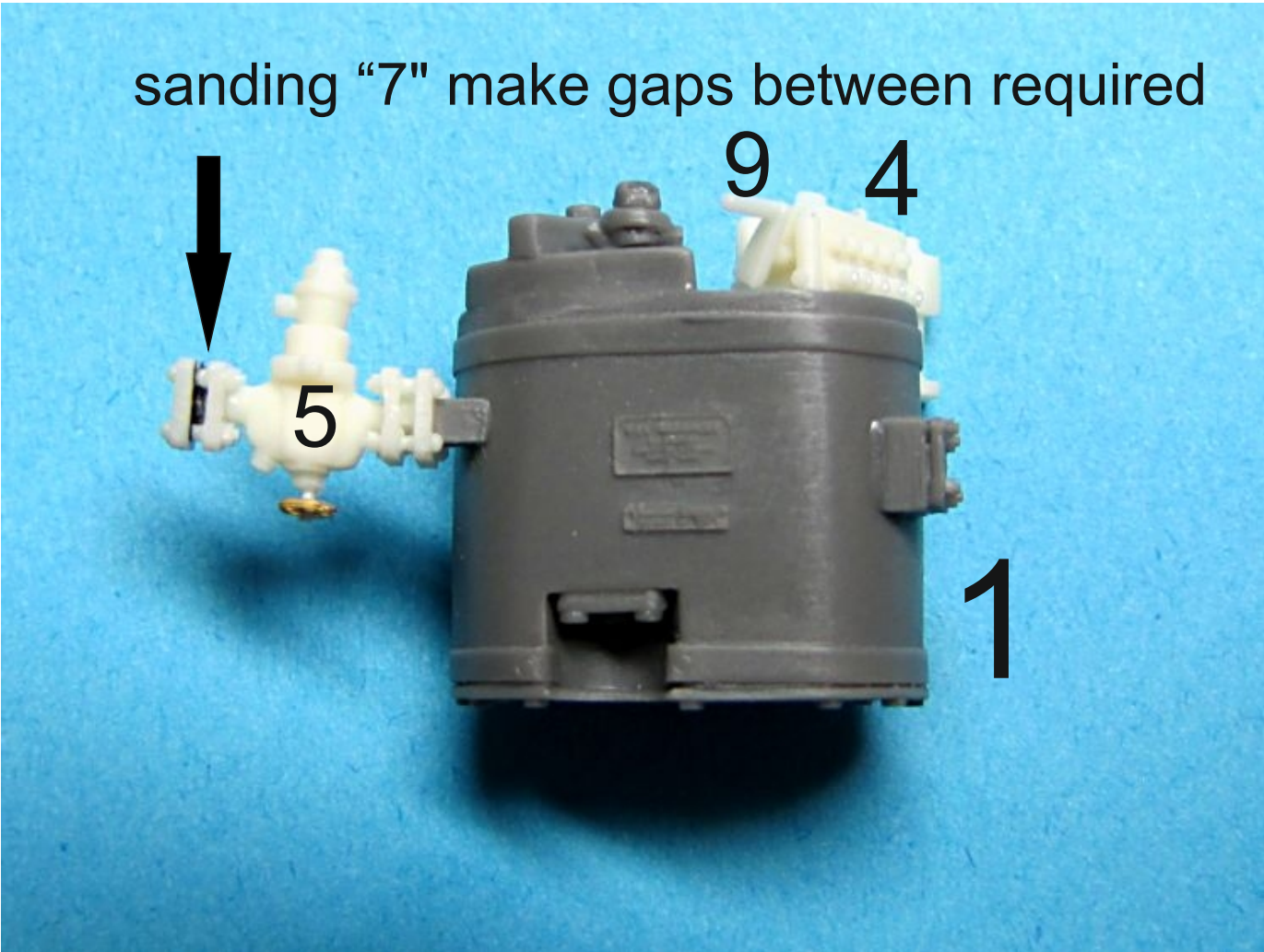
Steam part with grease pump and pressure controller
