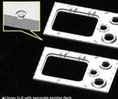
• Upper hull with separate engine deck • Two types of engine-deck hatch
