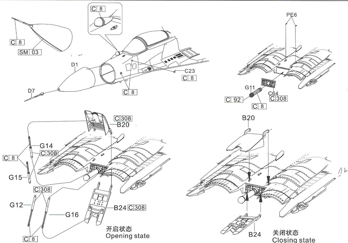
舱盖打开状态 Canopy opening state
