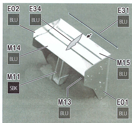
Rear Wing
