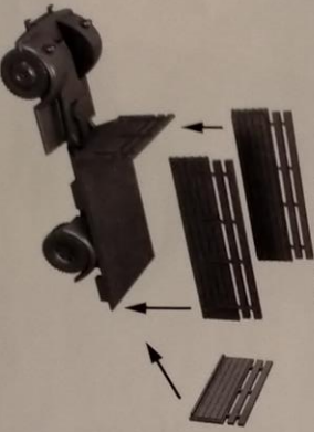
7. Assemble remaining rear panels
