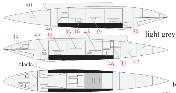
EMI Recce Pod for RAF(FGR.2)
