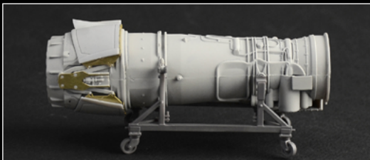
Removable RB.199 Engine with special support trolley
