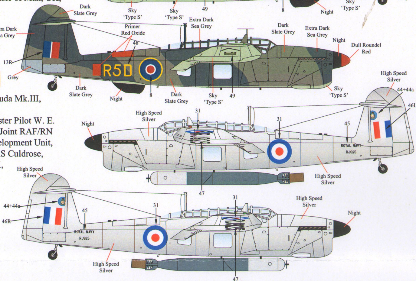
Fairey Barracuda Mk.I, PM949 '371/A'.
