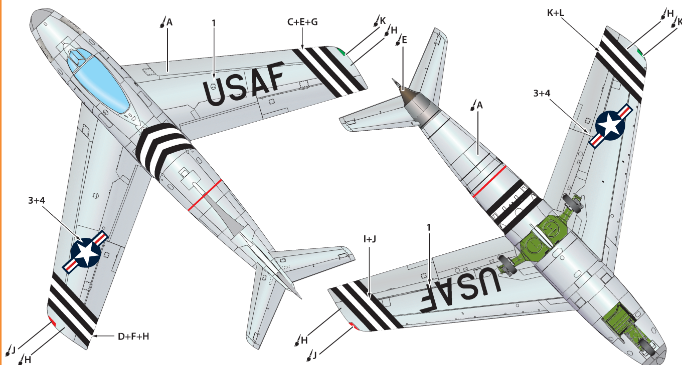
③ F-86A-5 s/n 48-261 "Scrambler" 1Lt Charles O Riester, Jr, 336th FIS K-14 Kimpo, Korea June 1951.
