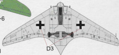
Horten Ho 229 V3 National Air and Space Museum Washington
