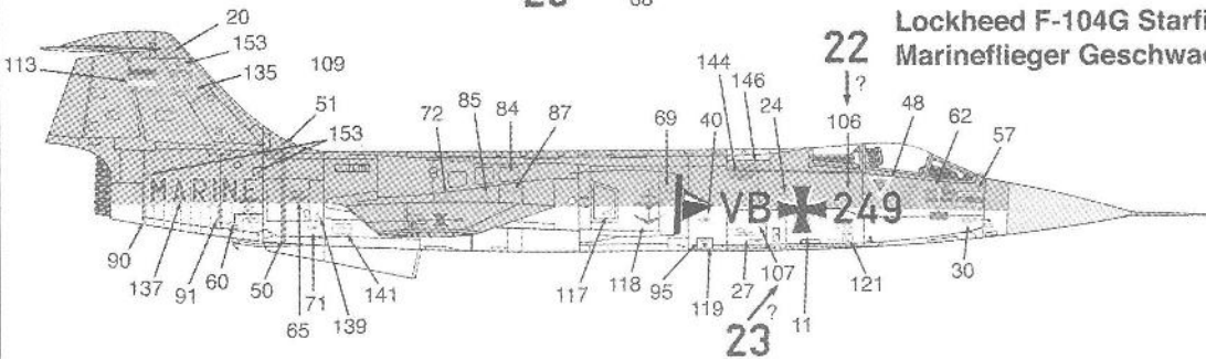
Lockheed F-104G Starfighter, German Navy Marineflieger Geschwader 1, Jagel, Germany "Bulls Eye 79" Weapons Meet 1979
