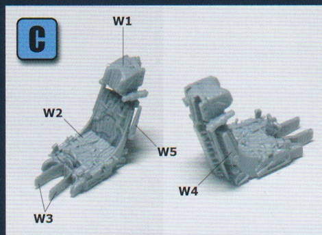
(C) K-36DM Ejection seat
