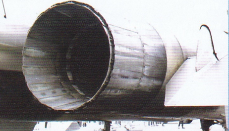
*AL-31F Engine nozzle
