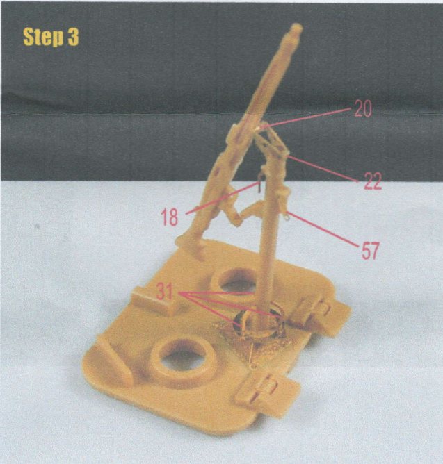
Jagdtiger Only
