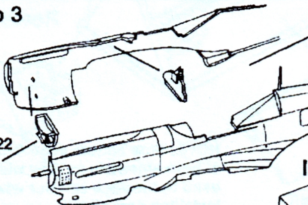
Fuselage Assembly
