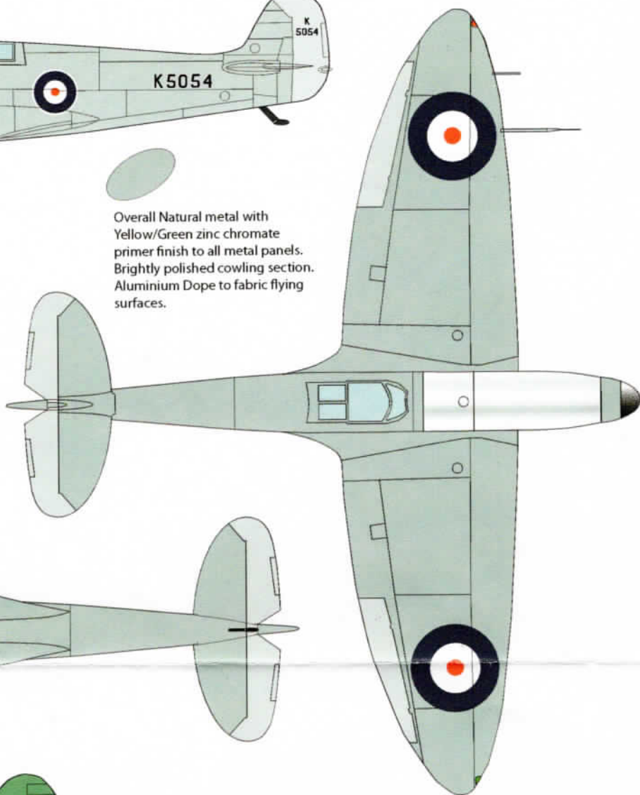
Scheme A K5054, Eastleigh Airport, 05 March 1936
