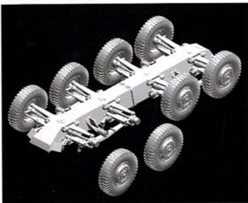
• Authentically recreated suspension and steering assembly
