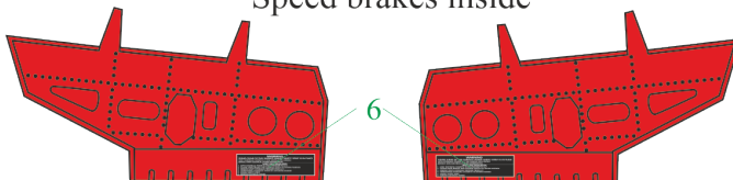
Speed brakes inside
