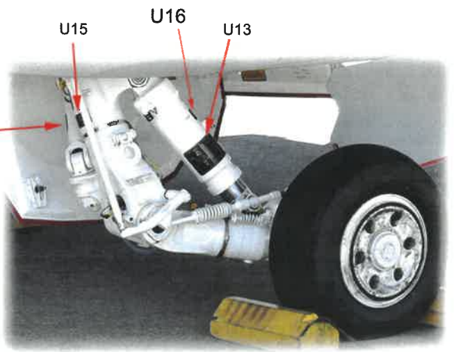
Port side undercarriage leg
