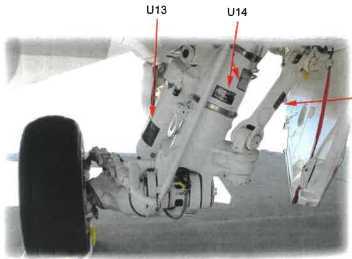
Starboard side rear undercarriage leg
