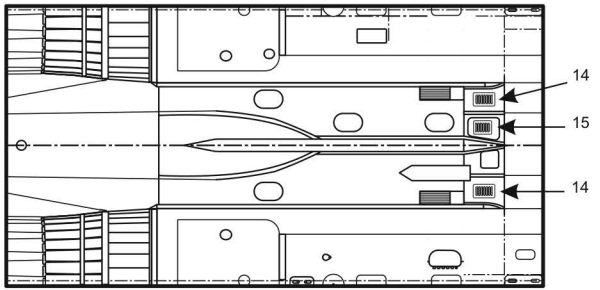
Su-35 bottom layout
