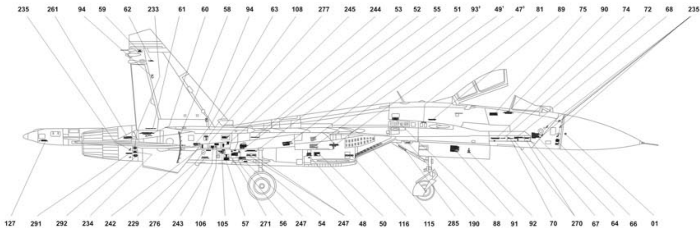
Su-27 from early, before 18-th, production batch, starboard view
