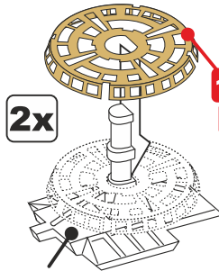
kit part F16.
