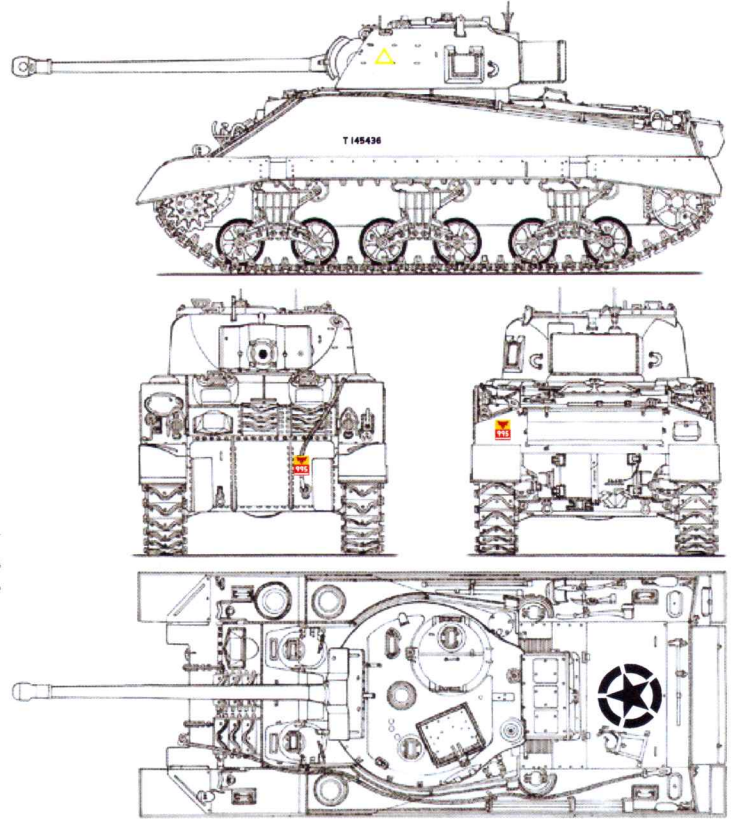
Sherman VC Firefly, 8th Armoured Brigade, 24th Lancers, A Squadron, Normandy, August 8th, 1944.
