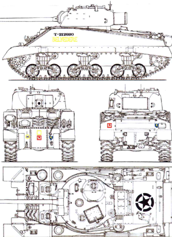
Sherman VC Firefly, "BELVEDERE" 27th Armoured Brigade, Staffordshire Yeomanry Regiment, B Squadron, Normandy, June, 1944.
