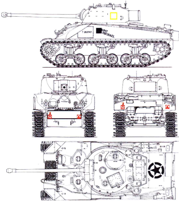
Sherman IC Hybrid Firefly "SAINT MICHAEL", 22nd Armoured Brigade, 5th Inniskilling Dragoon Guards, B Squadron, Normandy, 1944.
