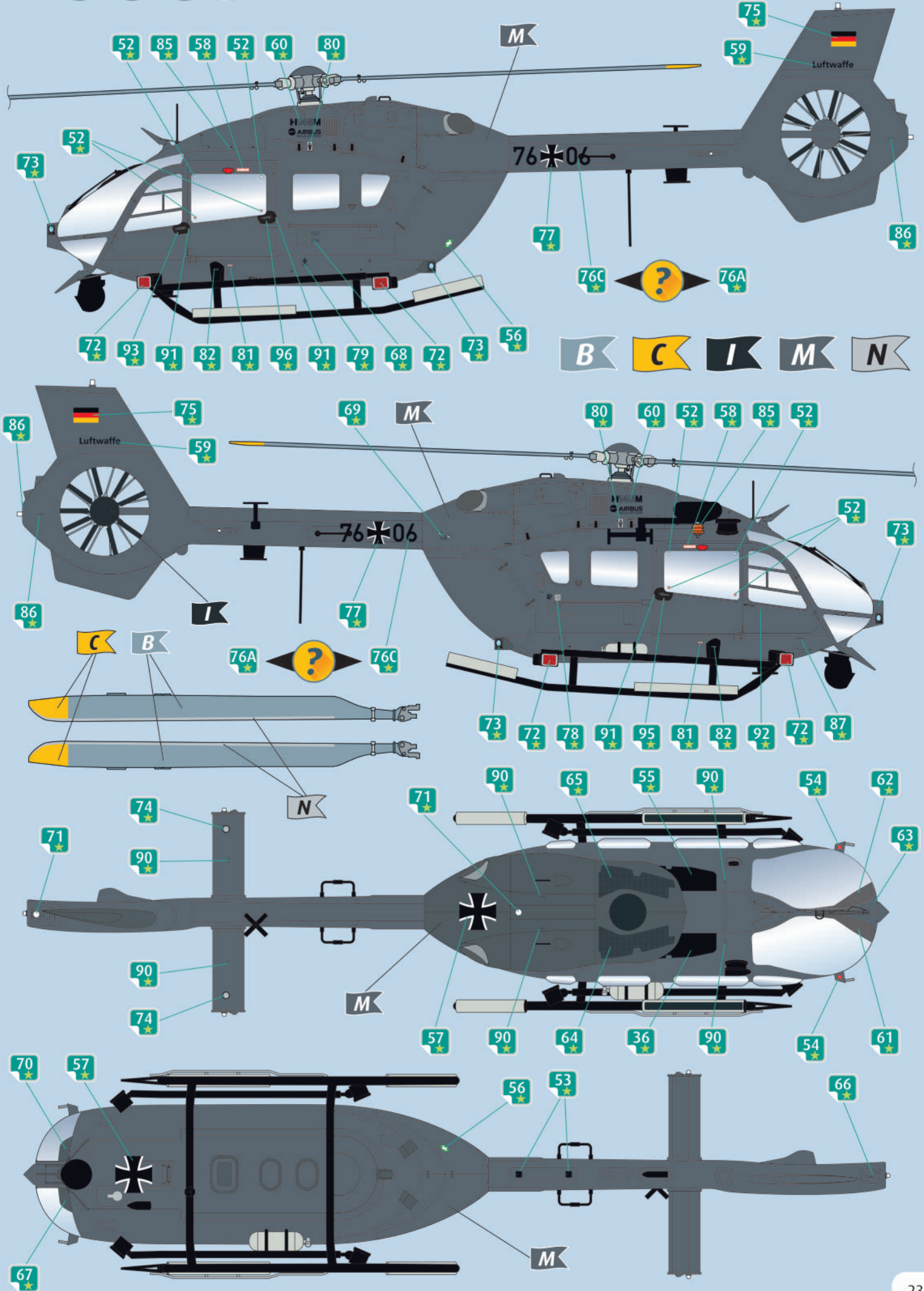
H145M, HSG 64, Laupheim, Germany, 2017 (surveillance version)
