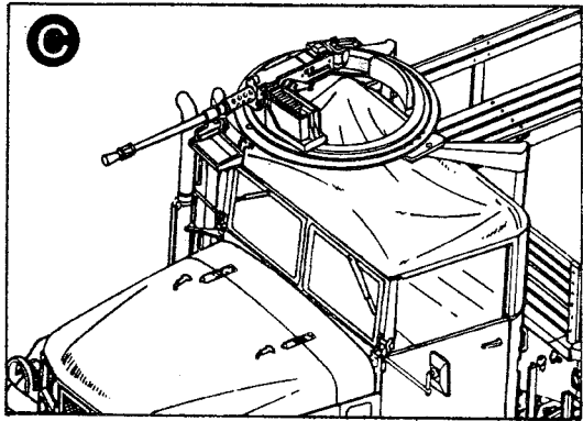
附機槍架時製作參考C步驟 STEP C: WITH MG MOUNTING
