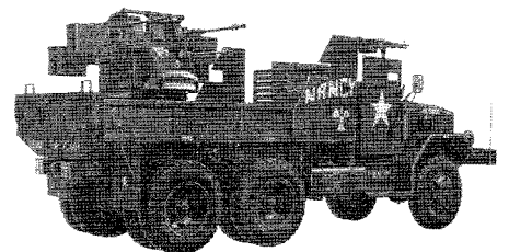
M35A1 GUN TRACK
