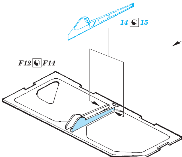
Left and right main wheel wells
