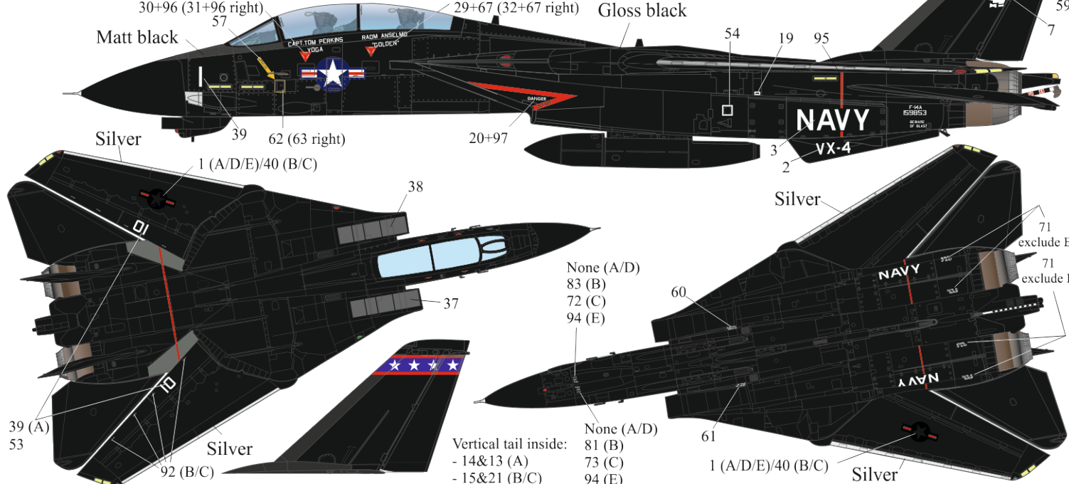
E. F-14A-90GR, Bu.No.159853. The typically "Black Bunny" paint scheme in VX-4, 1991.
