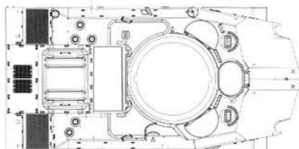
Upper hull
