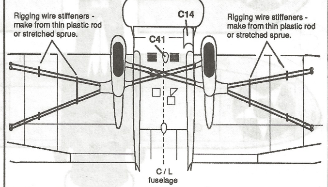
Rigging Diagram - Bottom View
